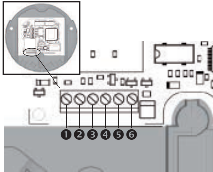
Terminal connections of the Datalogger
